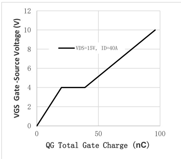
Fig.1 Gate-Charge Characteristics
