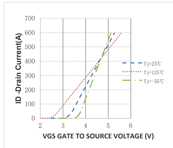
Figure 10. Transfer Characteristics
