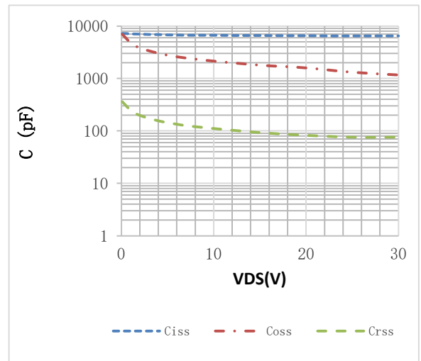
Fig.2 Capacitance Characteristics
